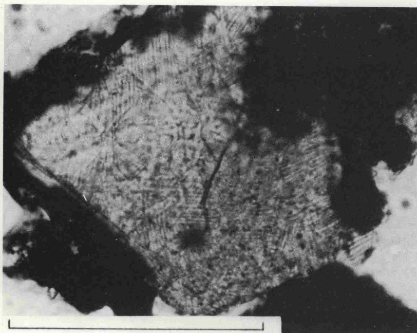
Fig. 1. Well-developed multiple sets of parallel shock lamellae in a pyroxene crystal. At least six separate sets can be distinguished. Fragment 318,512; plane polarized light; scale bar 0.1 mm.
