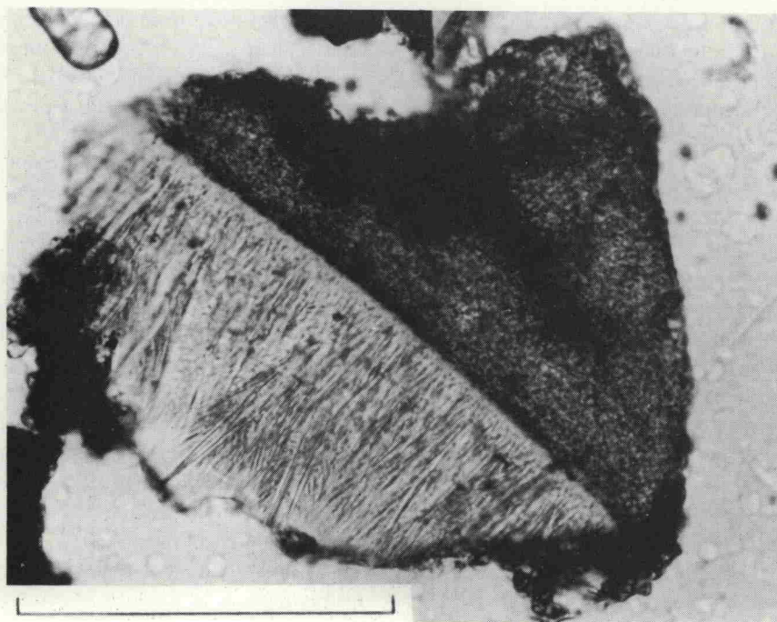
Fig. 2. Sharp contact between clear (plagioclase?) glass and a red-brown pyroxene(?) crystal which shows intense mosaic extinction and partial isotropization along dark veinlike regions. The plagioclase area, which was either maskelynite or shock-melted glass, is now partly devitrified to radiating and sheaflike plagioclase microlites. Fragment 318,362; plane polarized light; scale bar 0.1 mm.
